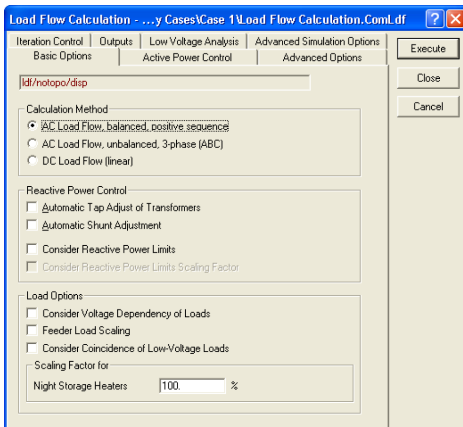
Fig. D.11: The load flow command dialogue
