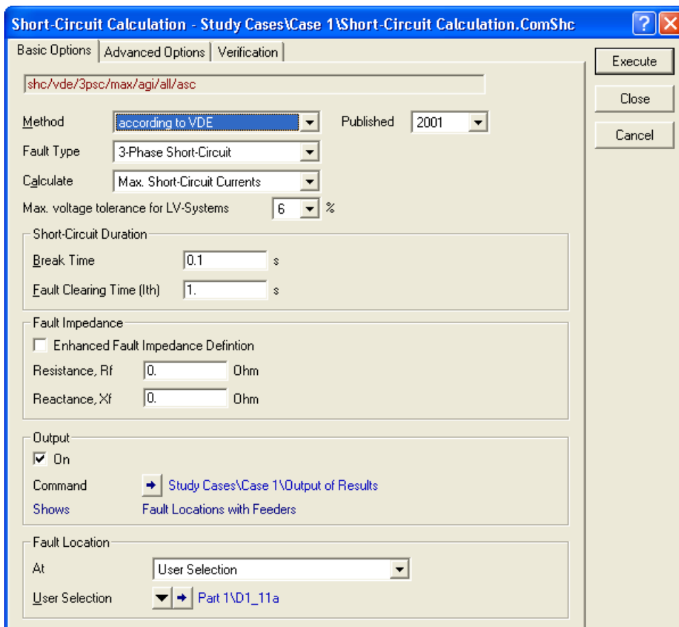
Fig. D.15: The short-circuit command dialogue
