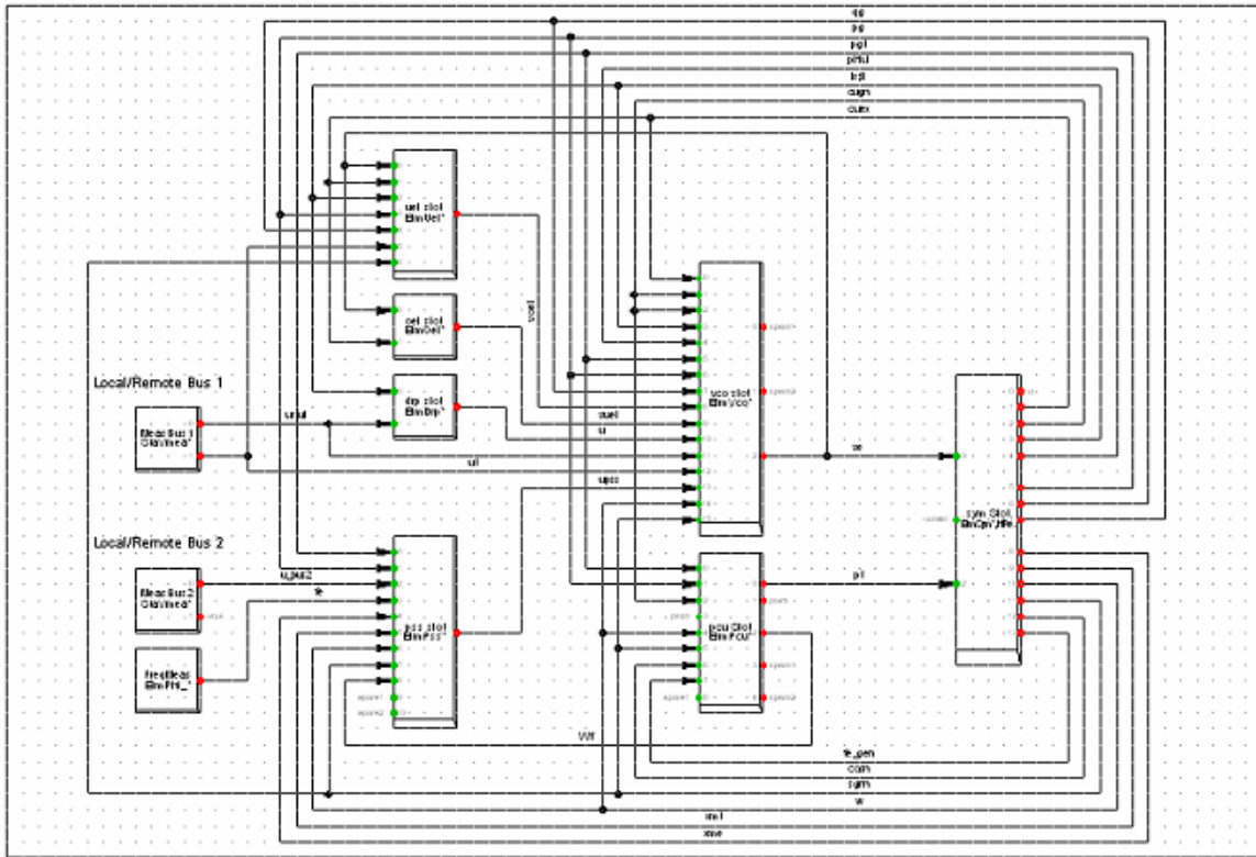
Fig. I.1: Composite Frame for synchronous machine
