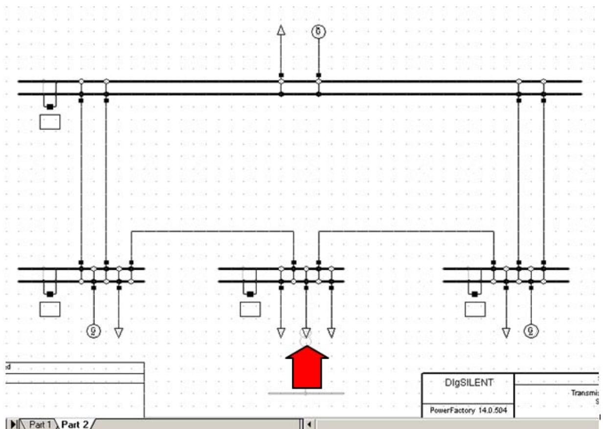
Fig. G.2: Transmission grid single line diagram (Part 2). Middle load representing the distribution load
