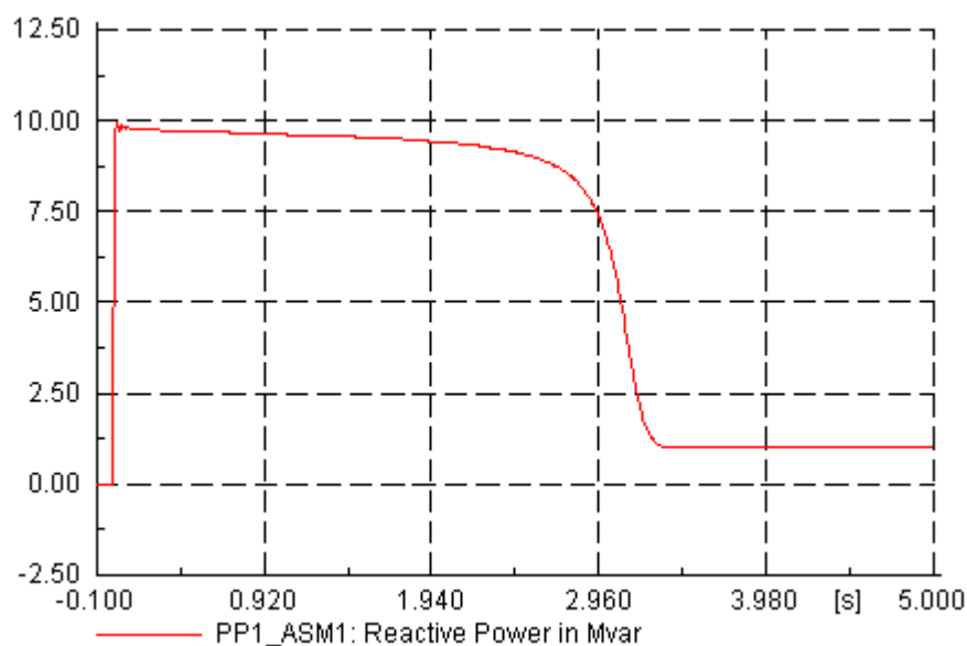
Fig. H.1: Reactive power demand during startup
