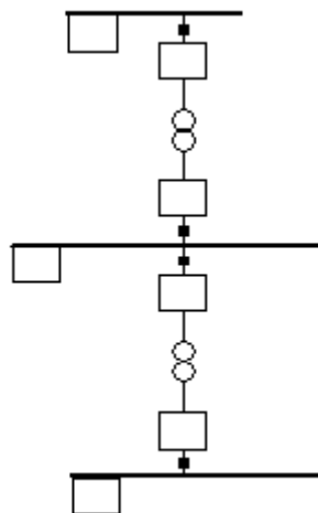
Fig. D.5: Three substations with single busbar systems and two transformers
