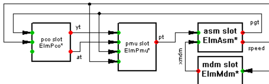
Fig. H.2: Composite Frame for asynchronous machine
