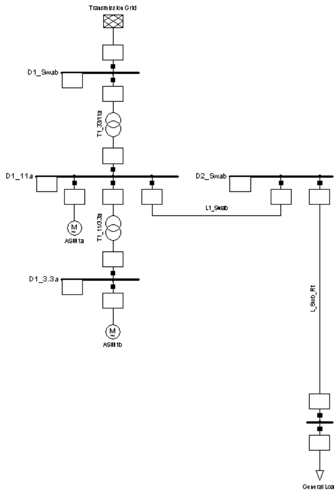
Fig. E.2: New cable, short terminal and load
